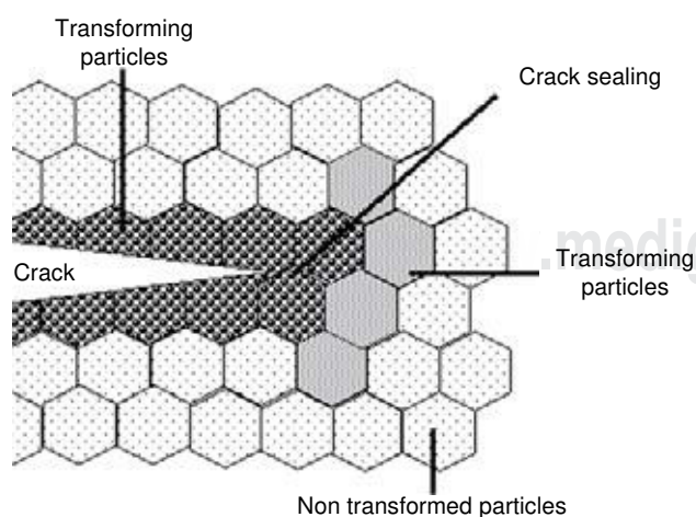
Figure 1. Representation of stress-induced transformation resistance process.
