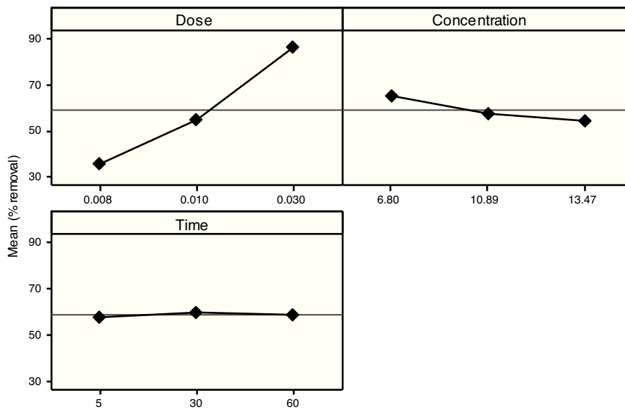
Fig. 6. Mean removal efficiency plotted against different factor levels.
