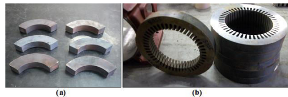
Fig. 11. Machine stator (a) parts compacted and sintered, (b) parts machined with grooves.
