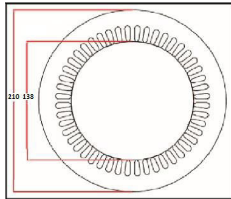
Fig. 2. Schematic of the stator core (dimensions in millimeters).
