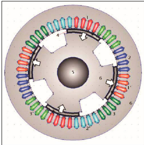
Fig. 6. Cross section of the machine.
