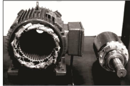
Fig. 1. Three-phase induction motor 10 HP partially disassembled.
