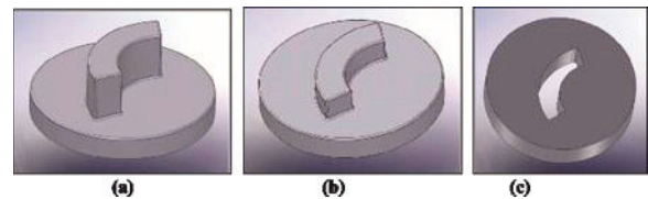
Fig. 8. Design of die for simulation (a) lower puncture (b) upper puncture (c) cavity.
