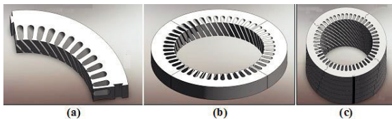
Fig. 7. (a) Segment, (b) block, and (c) set of six blocks.
