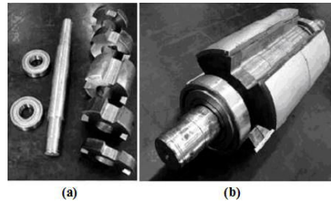
Fig. 10. (a) Pieces of rotor core developed (b) rotor developed with magnets fixed.
