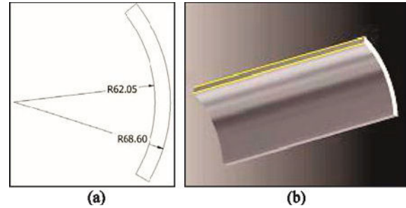
Fig. 4. (a) Dimensions of the cross section; (b) sketch in 3D.
