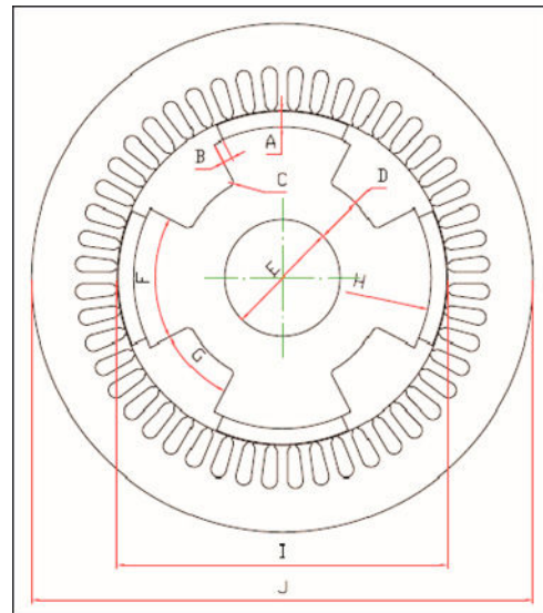
Fig. 5. Rotor quotas in cross-section.
