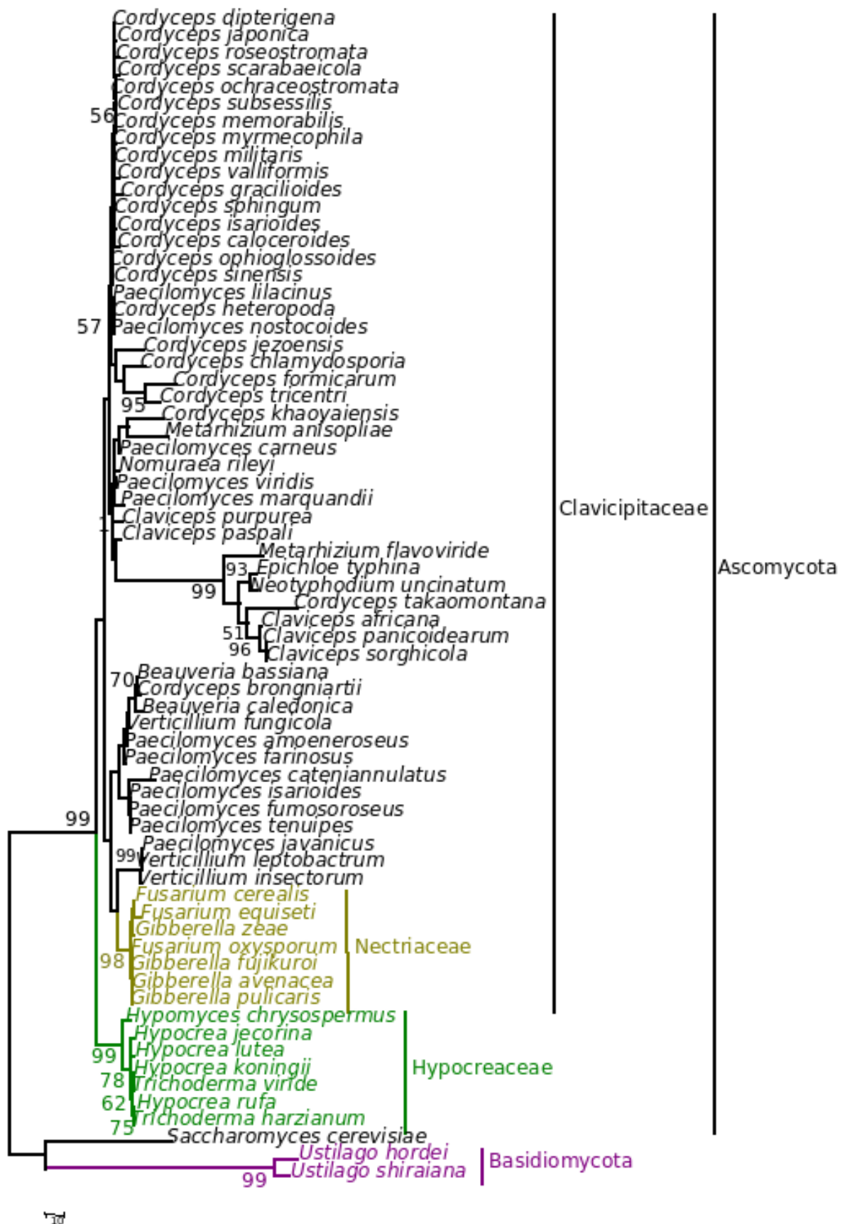
Figure 7. Consensus phylogenetic tree derived for the same data set as in Figure 1 derived by maximum parsimony analysis. Component tree statistics: tree length ( L ) = 574; consistency index (CI) = 0.0721; retention index (RI) = 0.818.
