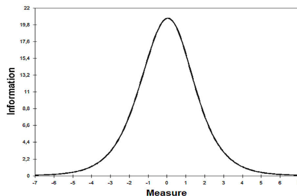
Figure 2 – Test information function of grandiosity dimension items set.
