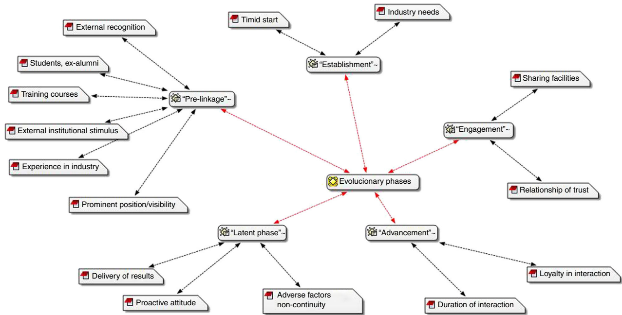
Fig. 1. Evolutionary phases.
