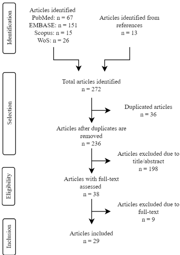
Figure 1 PRISMA flowchart.
