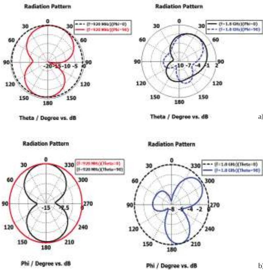
Figure 8. Radiation pattern for the main angles, a) Theta variation, b) Phi variation
