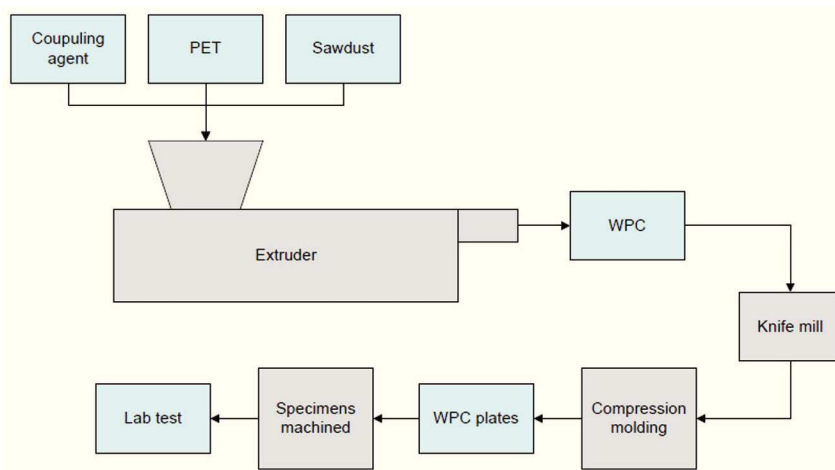
Figure 1. Description of the manufacturing process of the specimens
