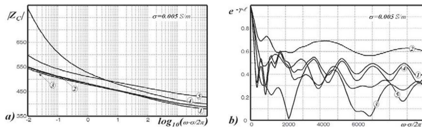
Figure 10. Frequency behavior of propagation modal functions, a) characteristic impedance Z_C and b) propagation function e^{-\gamma l}
