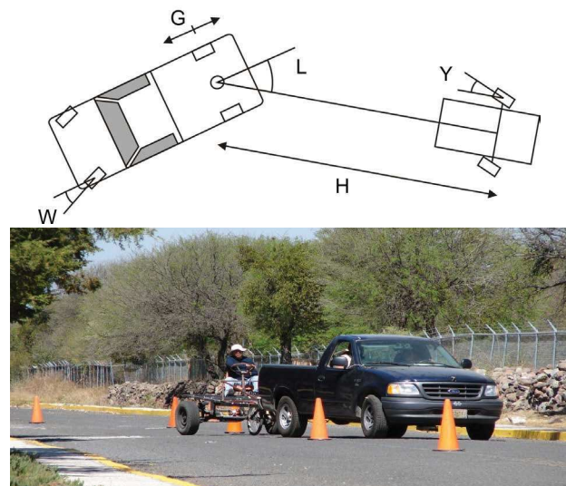
Figure 1. Experimental vehicle
