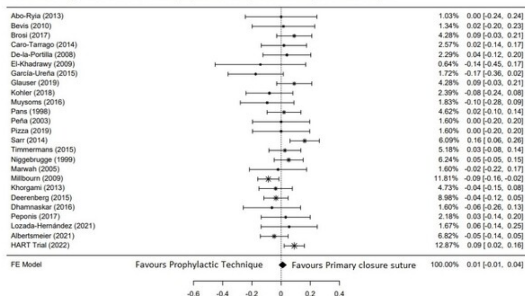
Forest Plot: Surgical Site Infection in Prophylactic techniques Vs Primary closure technique
