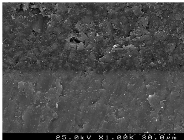
Fig. 3 – SEM photograph of resin–enamel interfaces with Transbond™ XT (G2) observed at x1000.
