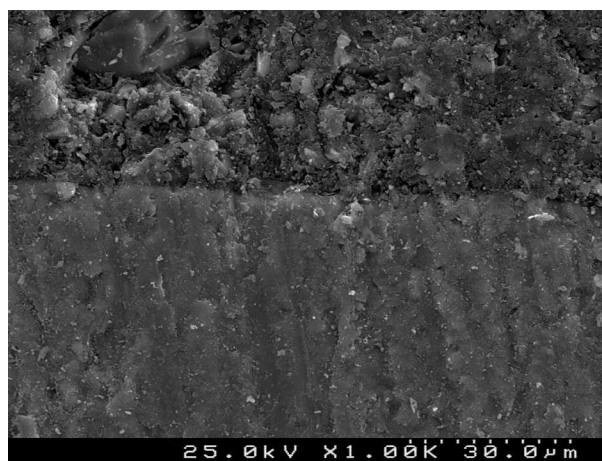
Fig. 4 – SEM photograph of resin–enamel interfaces with Transbond™ Plus Self-Etching Primer with Transbond XT (G3) observed at x1000.
