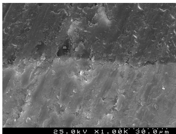
Fig. 5 – SEM photograph of resin–enamel interfaces with Heliosit® Orthodontic (G4) observed at x1000.
