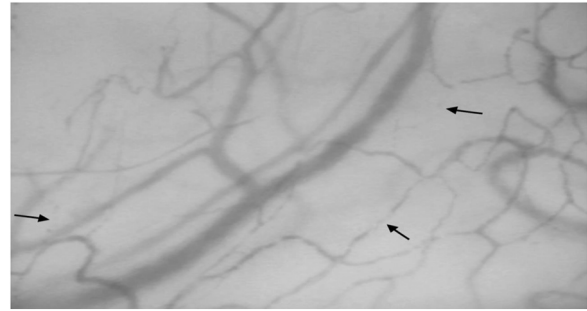
Fig. 1 – Sublingual microcirculatory imaging by Sidestream dark-field (SDF) in a patient with systemic sclerosis. Arrows depicts stopped and intermittent blood flow in vessels <20 \mu\text{m} of diameter.
