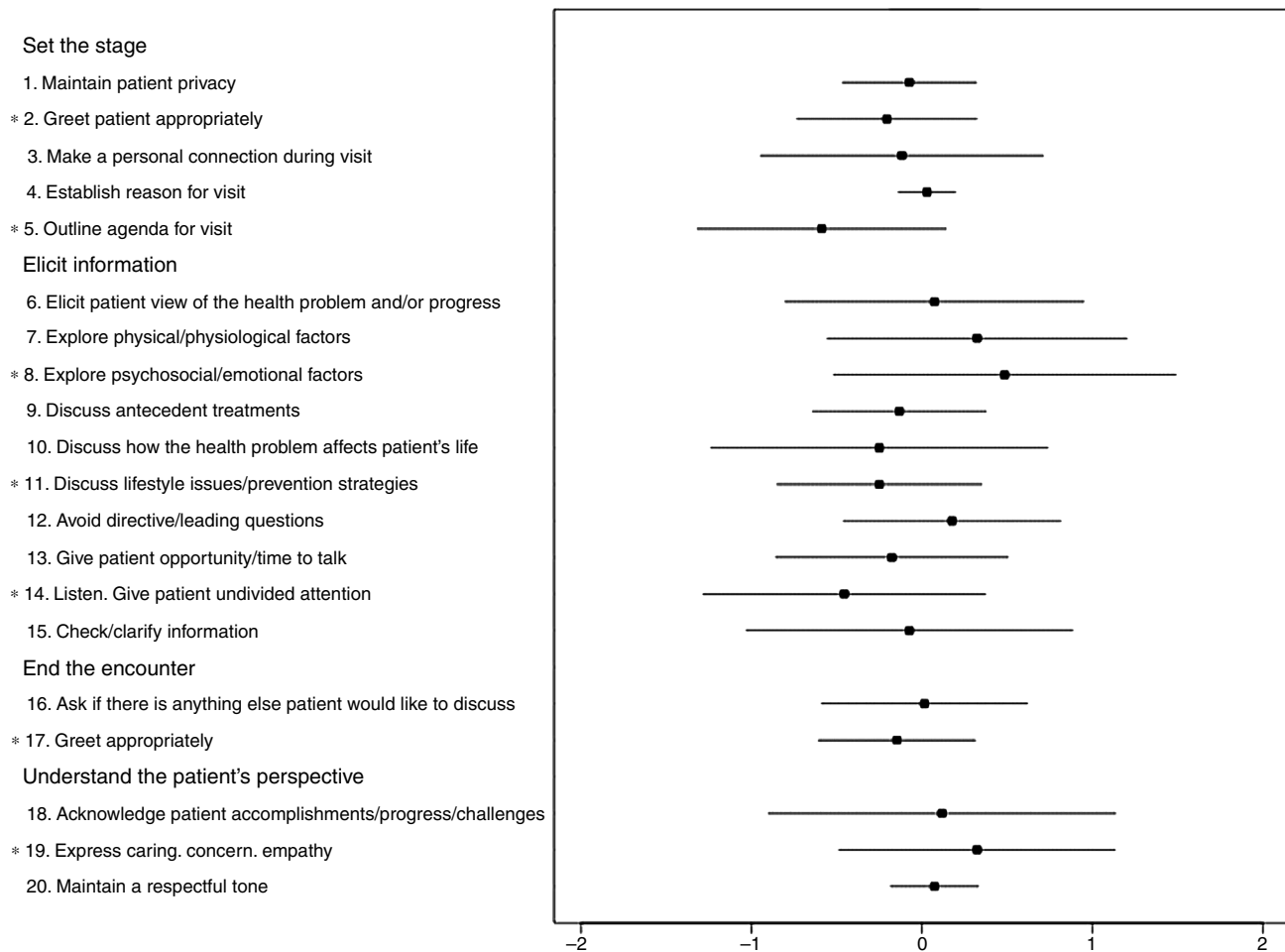
Fig. 2. Differences between mean values per item between T1 and T2 evaluations. * p < 0.0025 (paired samples t -test).
