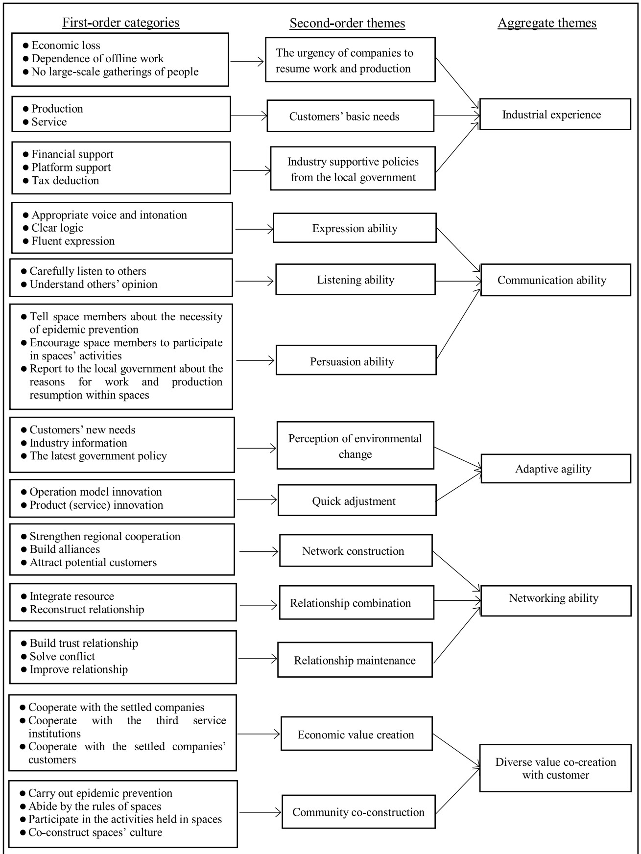
Fig. 1. Codification structure.
