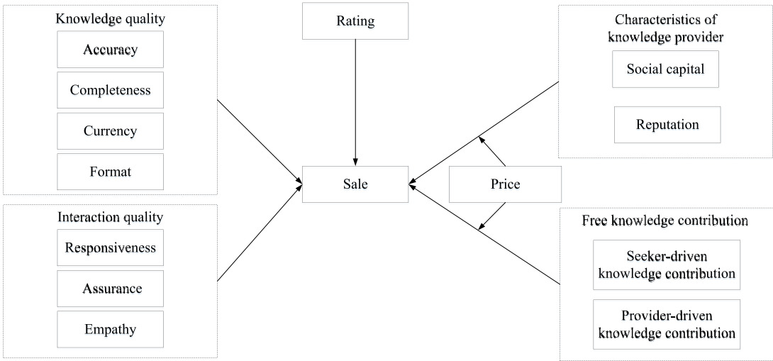
Fig. 1. Theoretical model.
