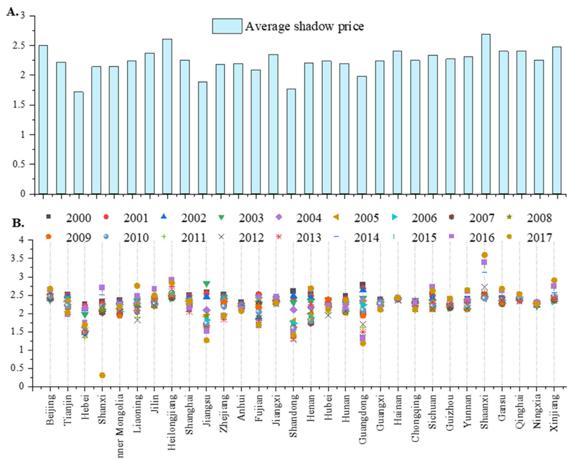
Fig. 5. Industrial carbon shadow prices across 30 Chinese provinces. (Unit: 10^4 yuan RMB per ton).
