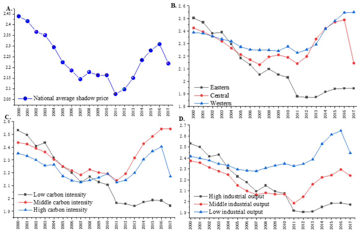
Fig. 4. Average industrial carbon shadow price in the whole nation and different regional groups. (Unit: 10^4 yuan RMB per ton).
