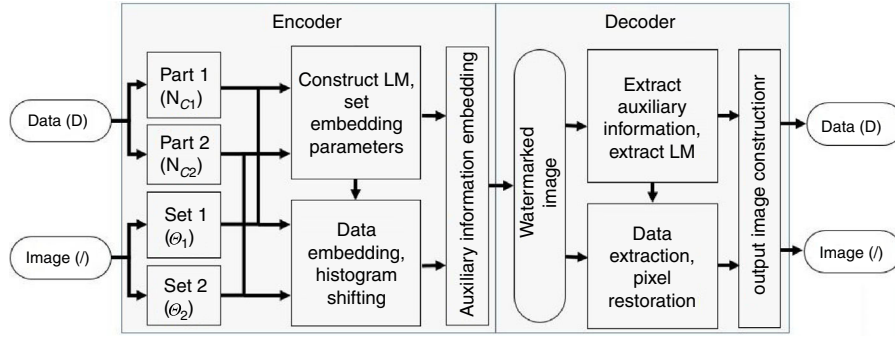
Fig. 4. System block diagram.
