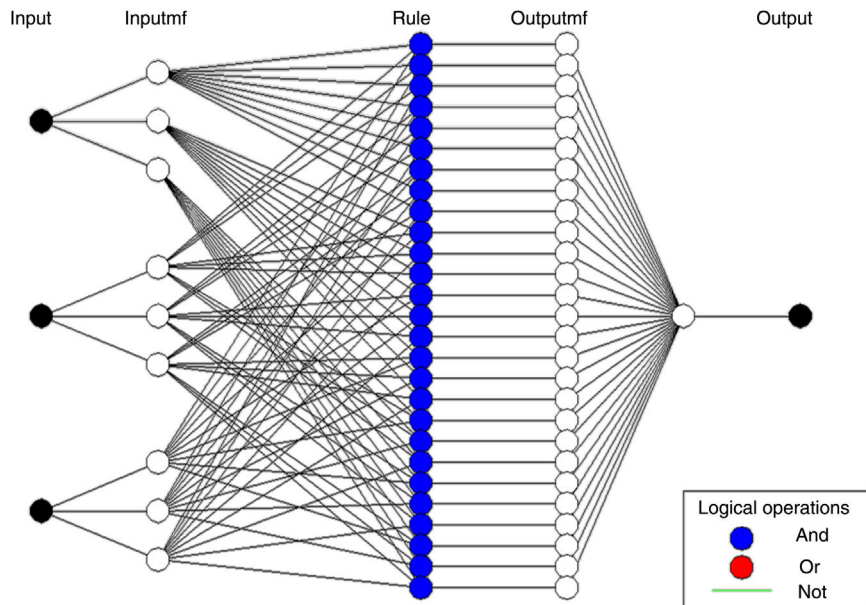
Fig. 2. Structure of adaptive ANFIS network.
