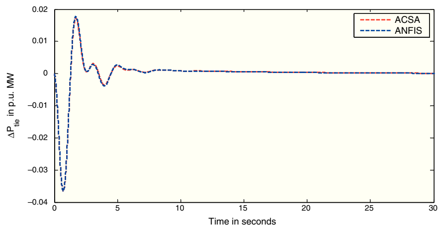
Fig. 5. Tie-line power deviation.
