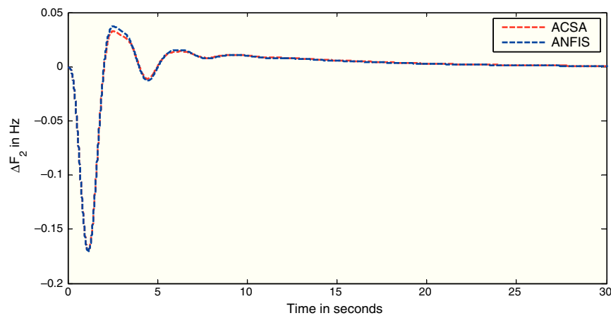
Fig. 4. Frequency deviation in area-2.
