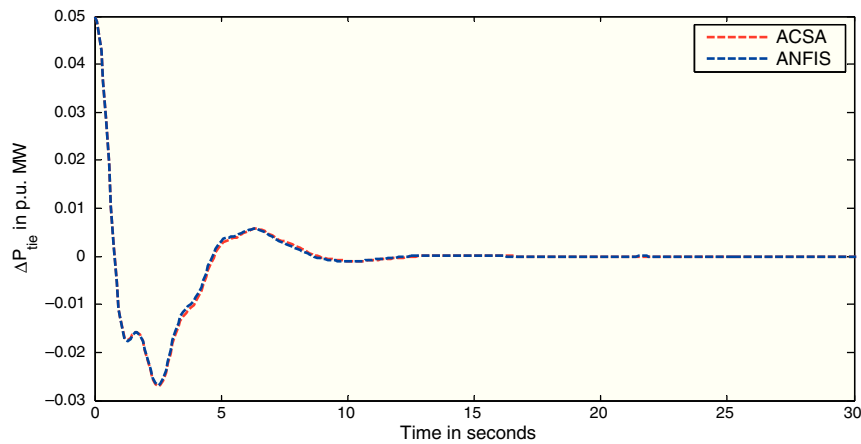
Fig. 20. Tie-line power deviation.
