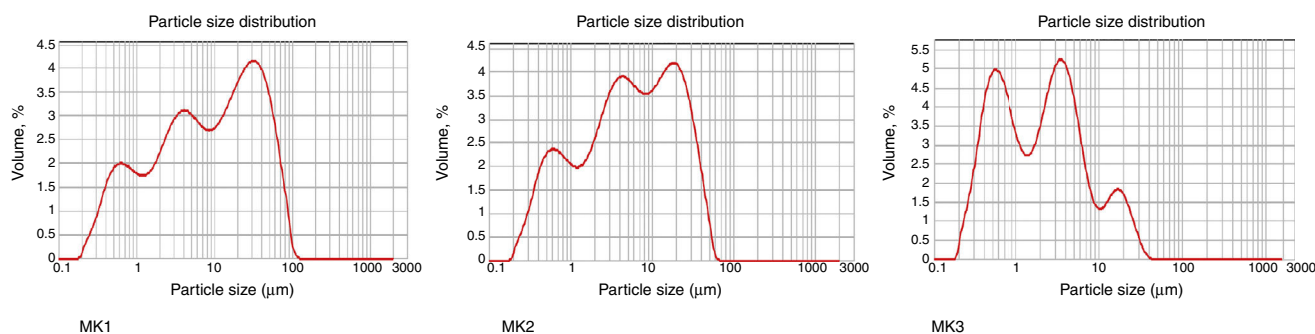
Fig. 2. The size distributions of metakaolin particles.
