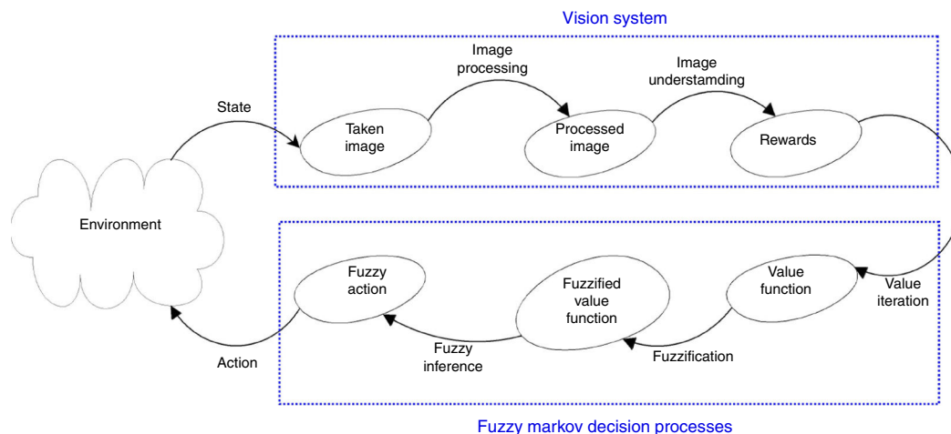
Fig. 8. Data flow.
