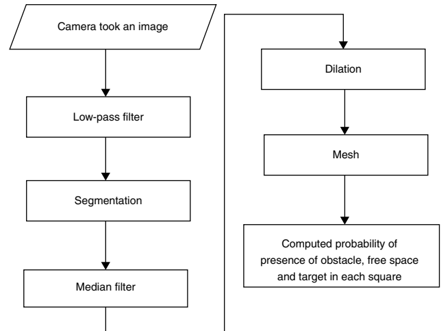
Fig. 3. Flowchart of vision system.
