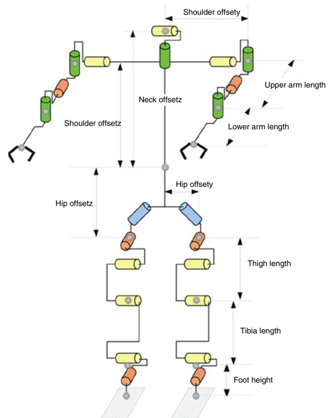
Fig. 11. Detailed kinematics of NAO. Wrist joint not represented (Gouaillier et al., 2009).
