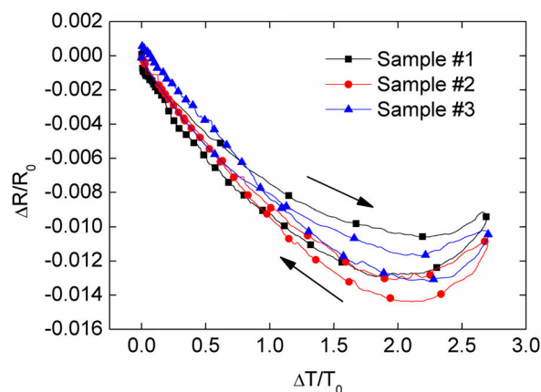
Fig. 11. Thermoresistive behavior of MWCNT/PSF samples characterized using the constructed oven.
