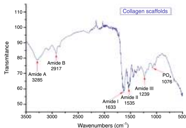
Fig. 6. Infrared spectra of CS where functional groups for amides (A, B, I, II, III) and phosphate ( \text{PO}_4 ) are identified.
