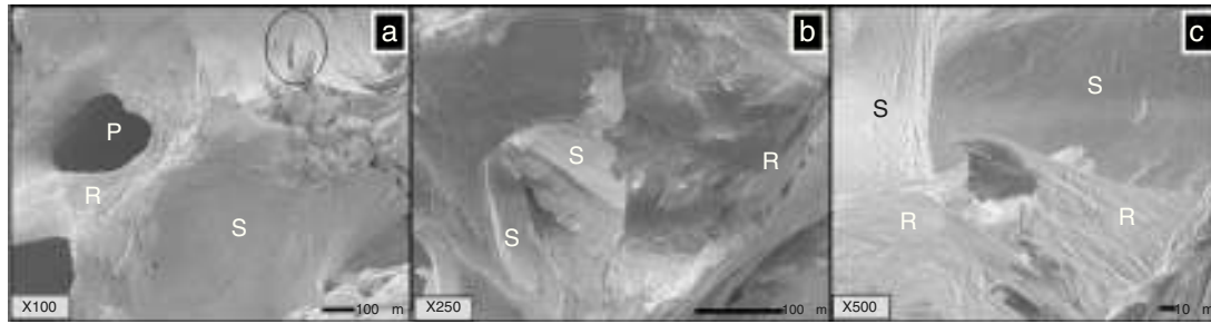
Fig. 3. (a) Bone matrix (BM) observed by SEM, pores are observed (P) and a smooth zone corresponding to the surface of HA (S), and a rough area (R) lacking of HA, corresponding to collagen fibers. SEM images of CS (b and c) showed two areas well identified; the smooth (S) surface corresponded with the area of HA which was removed by the demineralization process. The other zone was observed as rough (R) corresponding to collagen fibers. a: 100 \times , b: 250 \times , c: 500 \times .
