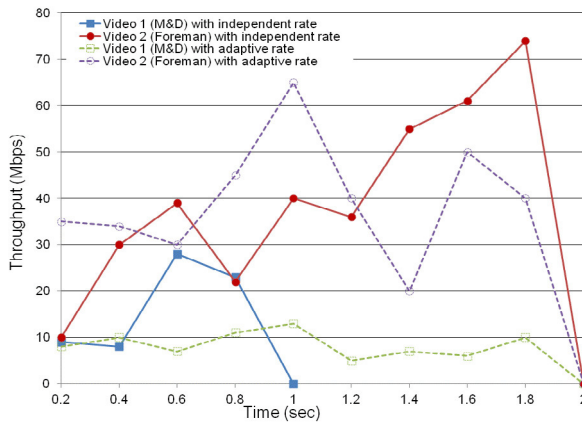
Figure 7. Distribution throughput on a source for two different video streams over a LAN.
