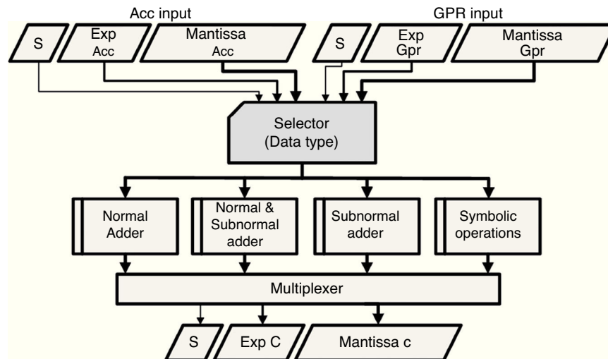
Fig. 8. Floating point adder-subtractor.
