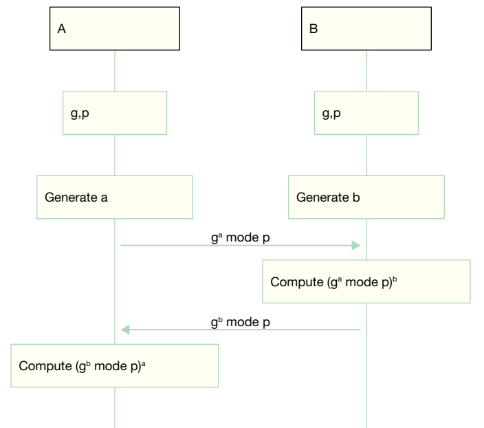
Fig. 9. Diffie-Hellman key agreement.
