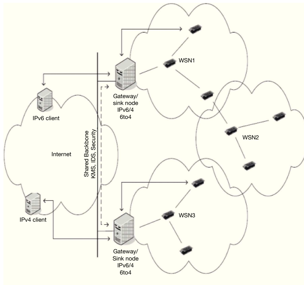
Fig. 2. Illustrates the operational scenario of SIMWSN [1].
