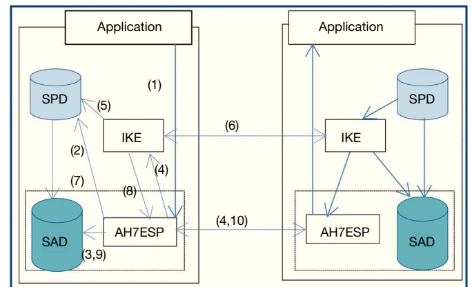
Fig. 7. IKE architecture.
