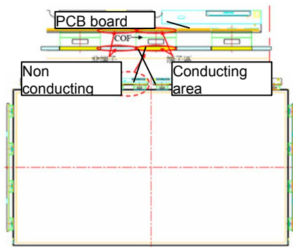
Figure 2. The conventional long bar ACF cutting process in the LCD panel.
