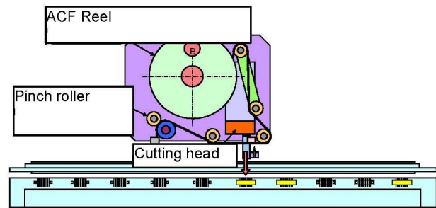
Figure 4. Short bar ACF cutting unit.
