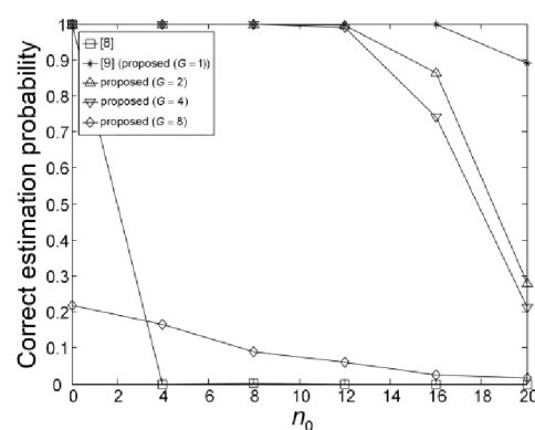
Figure 18. Correct estimation probabilities of the proposed and conventional schemes as a function of timing offset when SNR = -10 dB.
