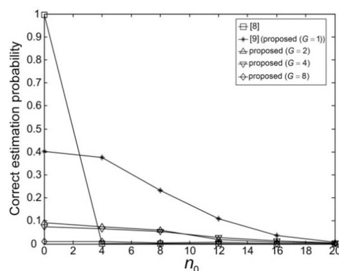
Figure 16. Correct estimation probabilities of the proposed and conventional schemes as a function of timing offset when SNR = -20 dB.
