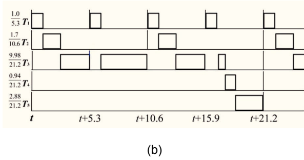
Figure 1. (a) Periodic and (b) jitterless schedule.
