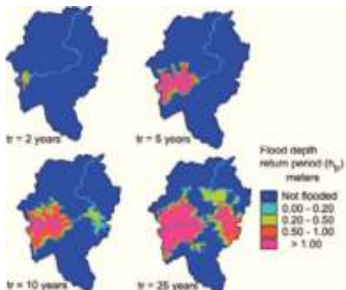
Figure 6. Example for flood risk analysis for several return periods in a watershed.
