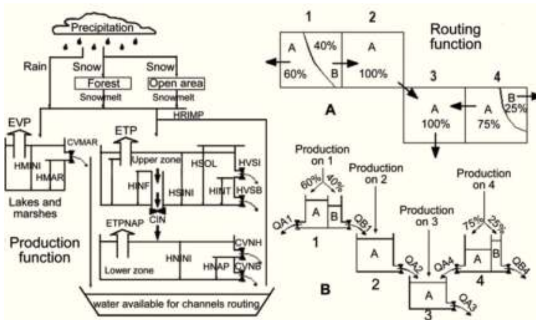
Figure 5. Schematic of a hydrological model for the process of rainfall runoff (modified from Eluch et al., 2009).
