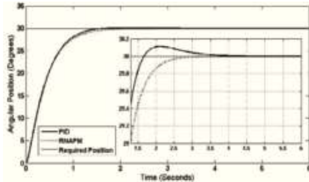
Figure 10. Behavior graph of PID and RNAPM control at 30^\circ angular position.
