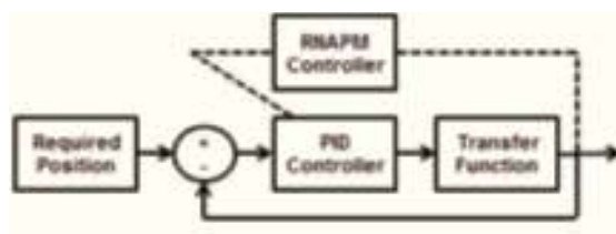
Figure 7. Diagram of the RNAPM control system.
