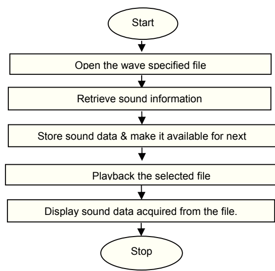
Figure 10. Flow chart of wave file player.vi.
