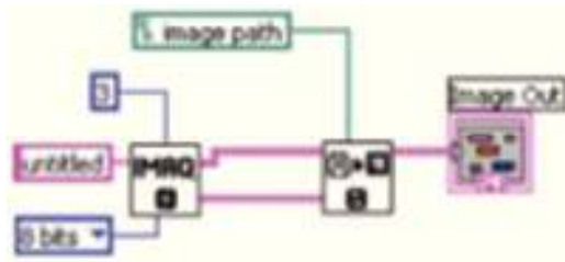
Figure 1. Image acquisition.
