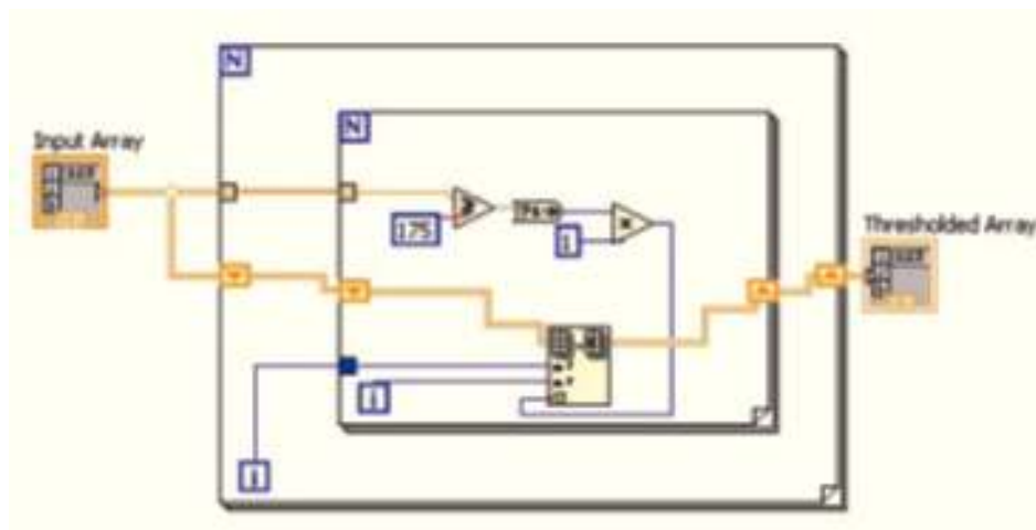
Figure 2. Binarization process.
