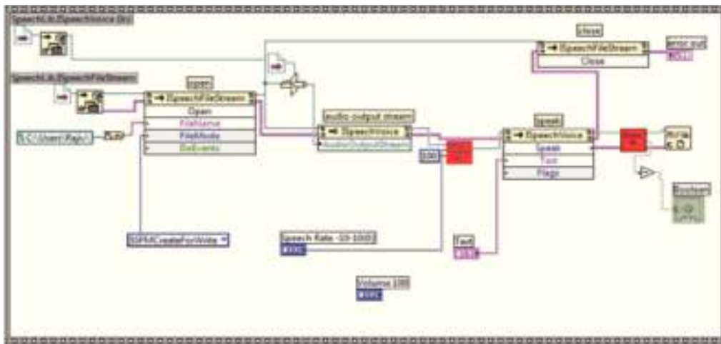
Figure 8. Text to speech conversions.
