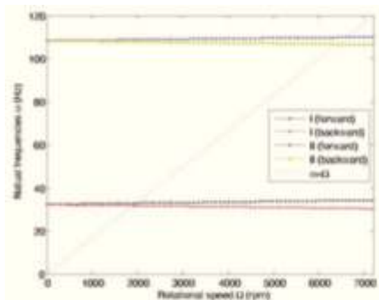
Figure 2. Campbell diagram.
