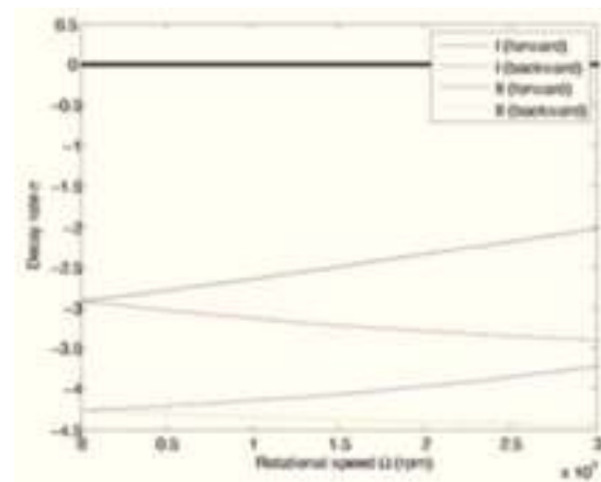
Figure 3. Decay rate.
