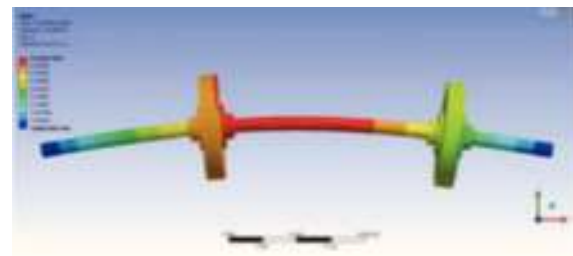
Figure 4. Modal shape related with the first natural frequency.
