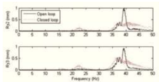
Figure 15. Experimental results in frequency domain.
