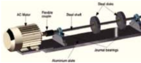
Figure 1. Rotor-bearing system.
