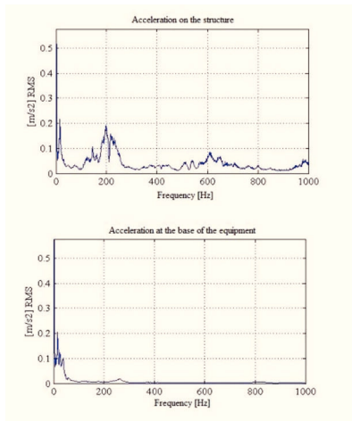
Figure 4. Typical spectra of vibrations on Z axis measured at the mobile unit structure and at the base of mammography equipment during transportation
