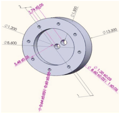
Figure 5. Sensor body.
