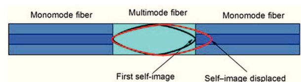
Figure 3. Displacement of the self-image in a MMI arrangement.
