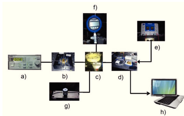
Figure 6. Proposed experimental arrangement.
