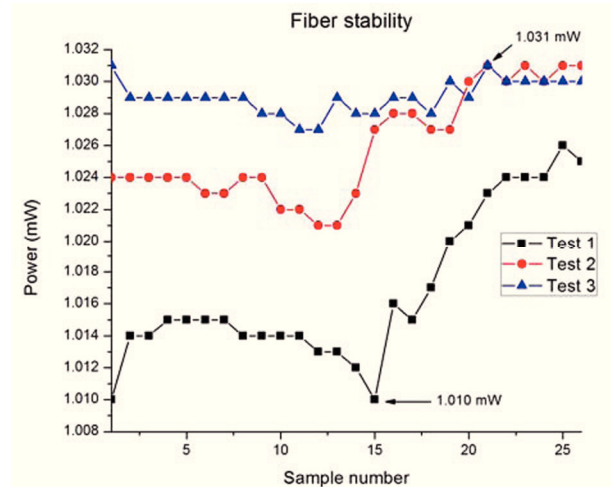
Figure 7. Fiber stability.
