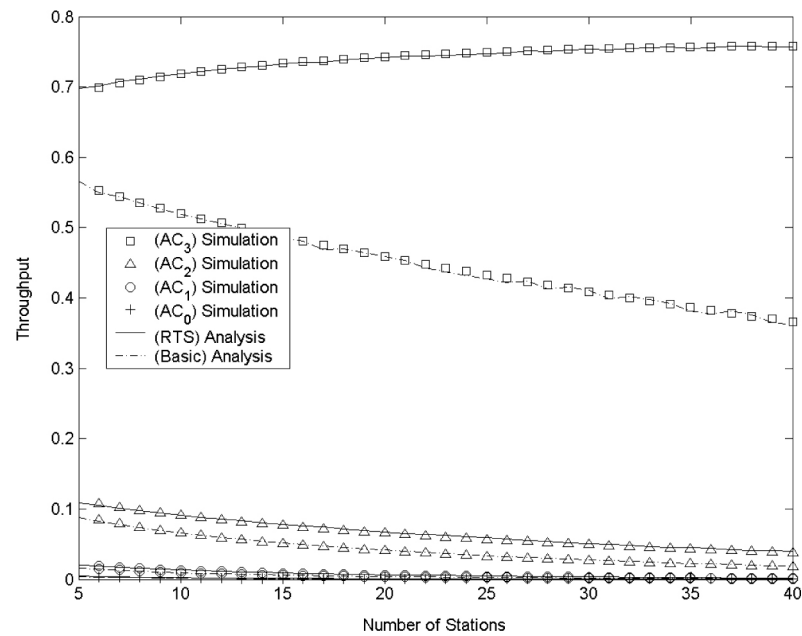
Figure 4. Saturation throughput: input parameter set II.
