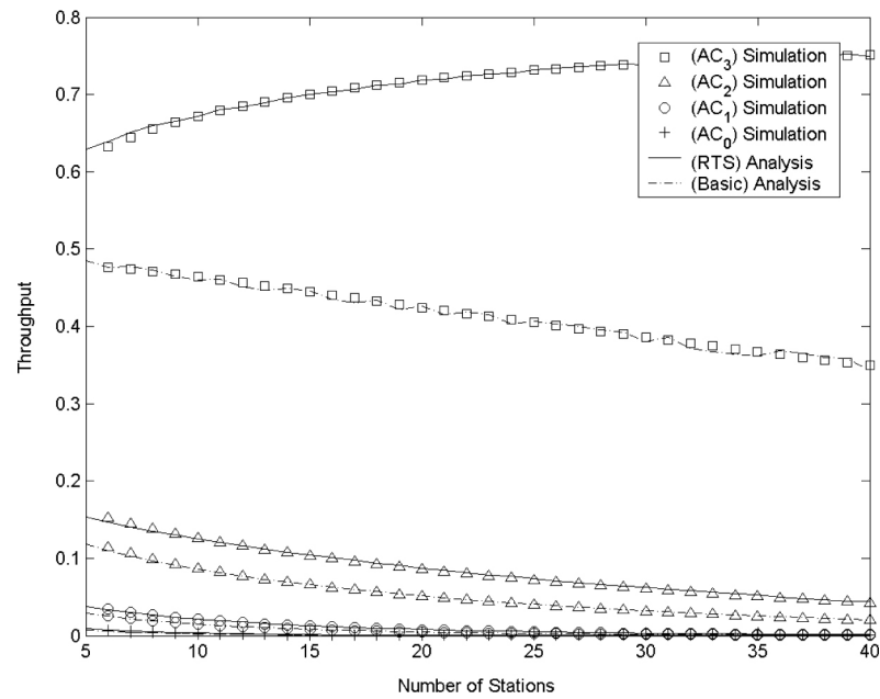
Figure 3. Saturation throughput: input parameter set I.
