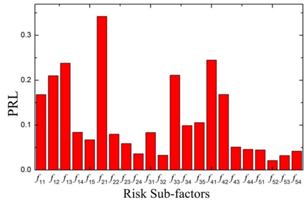
Figure 3. The histogram of PRLs of risk sub-factors in the general-assembling process A.
