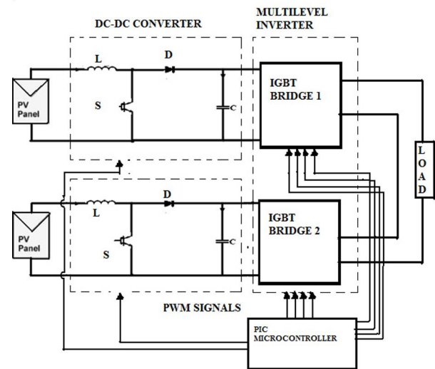
Figure 9. Experimental layout.
