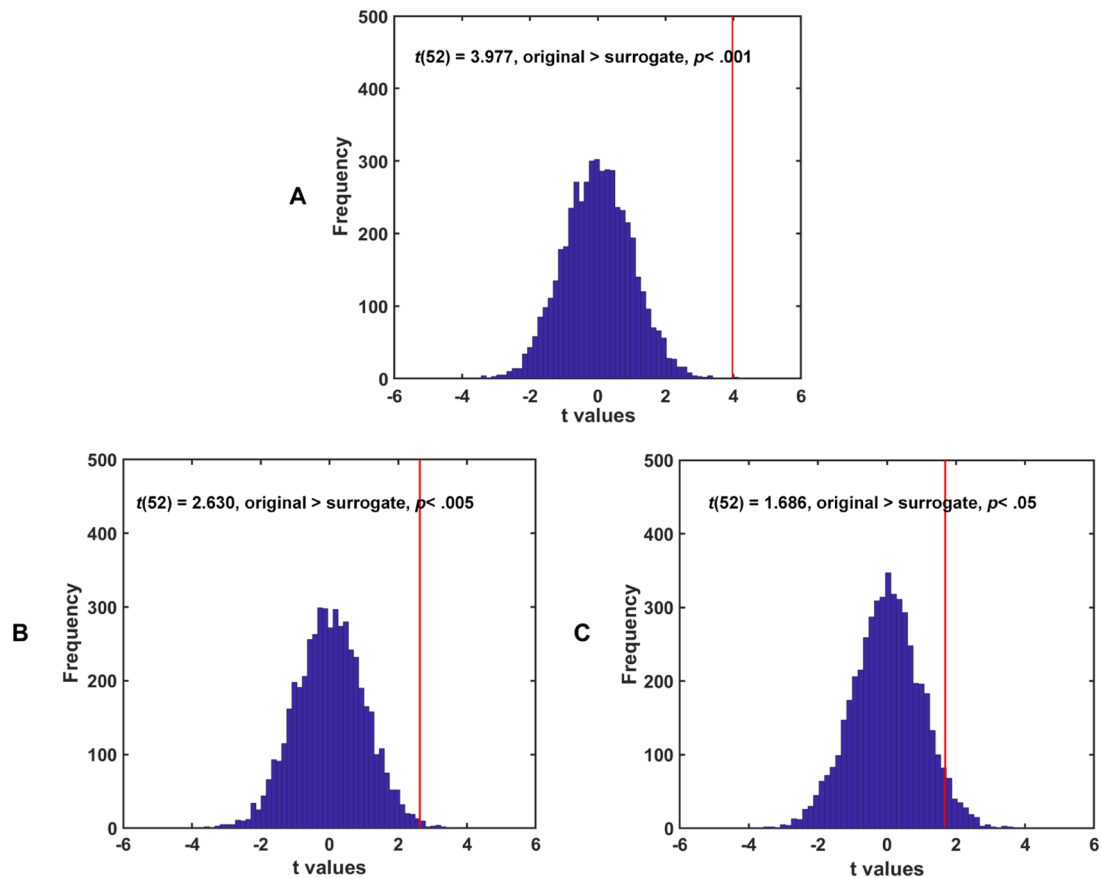
Fig. 2. The results of the permutation test. The effect (red line) in real dyads was significant within the 5 % area. The x-axis represents the t value, and the y-axis represents the number of the samples. (A. theta IBS permutation test results; B. beta IBS permutation test results; C. gamma IBS permutation test results).
