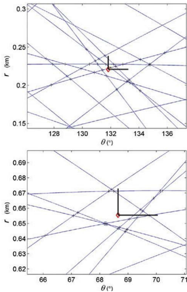
Figure 10. Close-up of the clusters used for determining the values of the parameters of alignments 1 (top) and 2 (bottom) in the example of imperfectly aligned data. The crosses represent the used intersections (sections of the cosenoid curves are shown for illustration purposes only; they are not used in the analysis), the parameter determinations are indicated by diamonds, and the circles show the locations of the true values.
