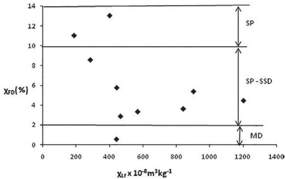
Figure 9. A schematic \chi_{if} - \chi_{fd}\% scattering diagram showing typical positions of samples from JMM.
