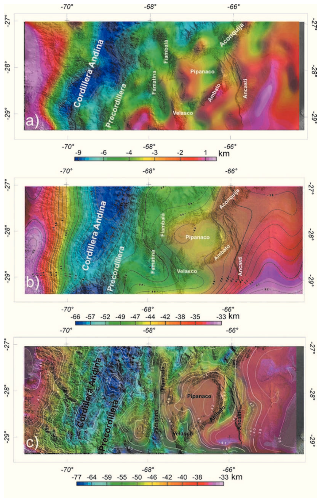
Figure 3. a) Top of basement, obtained by gravimetric inversion of the Bouguer anomaly map, based on the parameters in Chart 1. b) Crust-mantle depth obtained by gravimetric inversion of Bouguer regional anomaly. c) Isostatic model compensated on the Airy hypothesis of the crust-mantle boundary.
