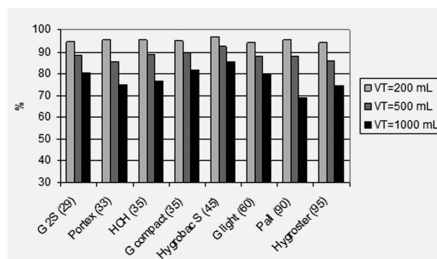
Figure 2 - Effect of tidal volume (200, 500 and 1000 mL) in the context of %RAH. The dead-space volume for each HME is shown in parentheses and the HME units are listed in order of increasing dead-space volume. Overall, the HME models differed slightly in terms of their ability to maintain absolute humidity levels, except when a high tidal volume was delivered. There was an inverse relationship between the efficiency of humidification and tidal volume. Hygrobac S was the HME model with the greatest %RAH.
