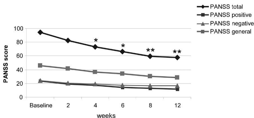
Figure 2 - PANSS – the mean change from baseline. PANSS: positive and negative syndrome scale, n = 17 , * p < 0.05 vs. baseline, ** p < 0.01 vs. baseline.
