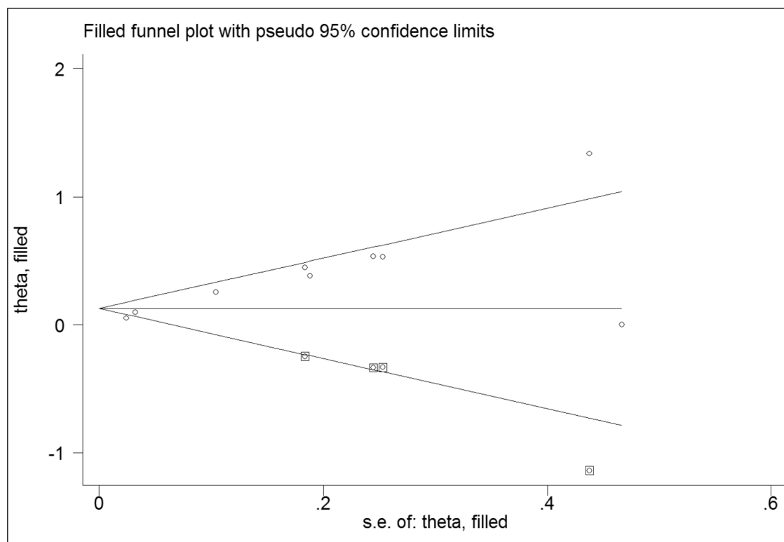
Figure 5 - Funnel plots adjusted with the trim and fill method for OS. Circles: included studies. Diamonds: presumed missing studies.
