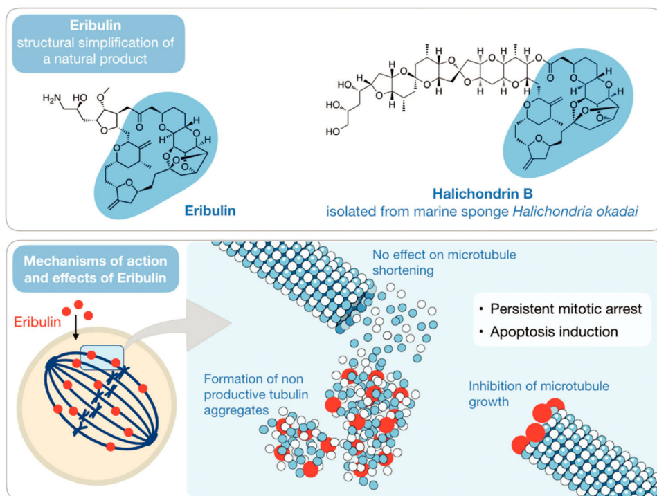
Figure 3 - Chemical structures of eribulin mesylate and the related natural product halichondrin B isolated from the sponge Halichondria okadai (top). A schematic representation of the mechanism of action of eribulin mesylate in cancer cells (bottom).
