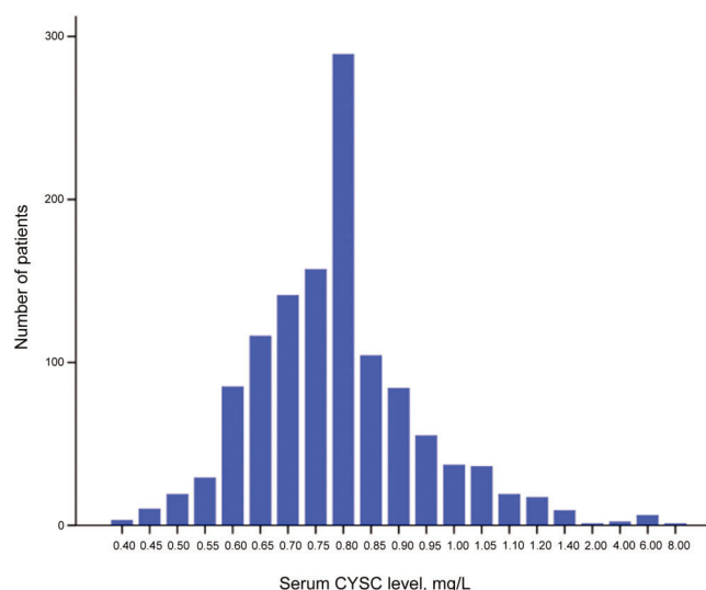
Figure 2 - The distribution of serum cystatin C levels.
