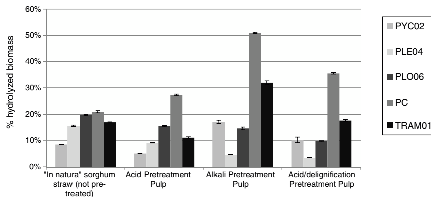
Fig. 1 – Saccharification of forage sorghum straw “in natura” (without pre-treatment) and of the pulps obtained from pretreatment according to Cardoso et al., 11 by crude extracts of fungi, P. chrysosporium PC, P. sanguineus PYC02, T. versicolor TRAM01, P. eryngii PLE04 e P. ostreatus PLO06, produced by SSF of forage sorghum straw.
