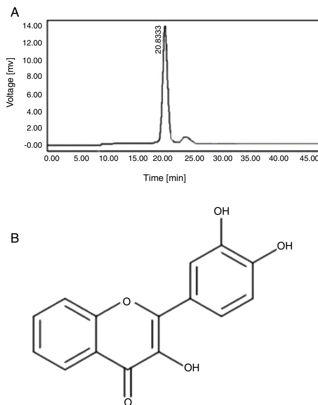
Fig. 6 – (A) HPLC fraction of CHF1; A single peak showing at RT 20.5 min. (B) Structure of 3,3',4'-Trihydroxyflavone; IR: 3336 cm -1 OH stretch, 1588 cm -1 , 1471 cm -1 aromatic ring stretching, 1416 cm -1 C=O stretch, 1195 cm -1 C–O–C stretch, 1007 cm -1 , 781 cm -1 , 637 cm -1 aromatic CH stretch., 1 H NMR (400 MHz, DMSO-d 6 , ppm): δ 5.35 (s 2 protons, phenolic OH) δ 6.87–8.07 (m, 7H, phenyl rings), 9.24–9.51 (s, 1H, OH proton). 13 C NMR (100 MHz, DMSO-d 6 , ppm): δ 115.73, 116.0, 118.57, 120.44, 121.75, 122.74, 124.79, 125.1, 133.77, 138.29, 145.52, 146.57, 148.06, 154.81, 172.9. LC-MS m/z 272 (M + ).
